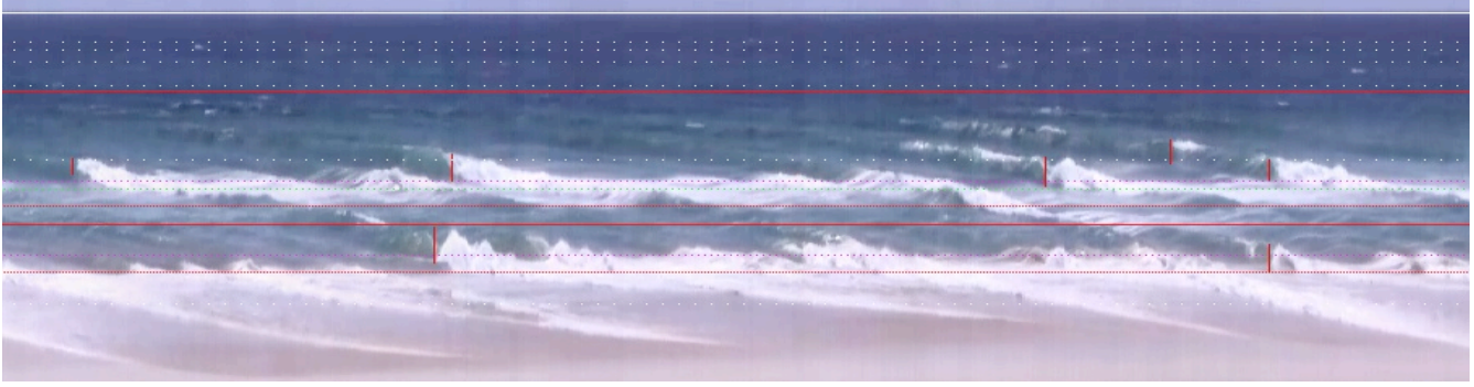
Figure 2: Section of timestack image with breakzones detected (between each solid and dotted horizontal red lines), swash zone (first horizontal dotted line in outer breakzone or green line), outer break point (second horizontal dotted line in outer breakzone or purple line) and measured breaking wave heights (vertical segments in red). The horizontal dotted white lines represent different distances while the solid white line represents the calculated horizon.
